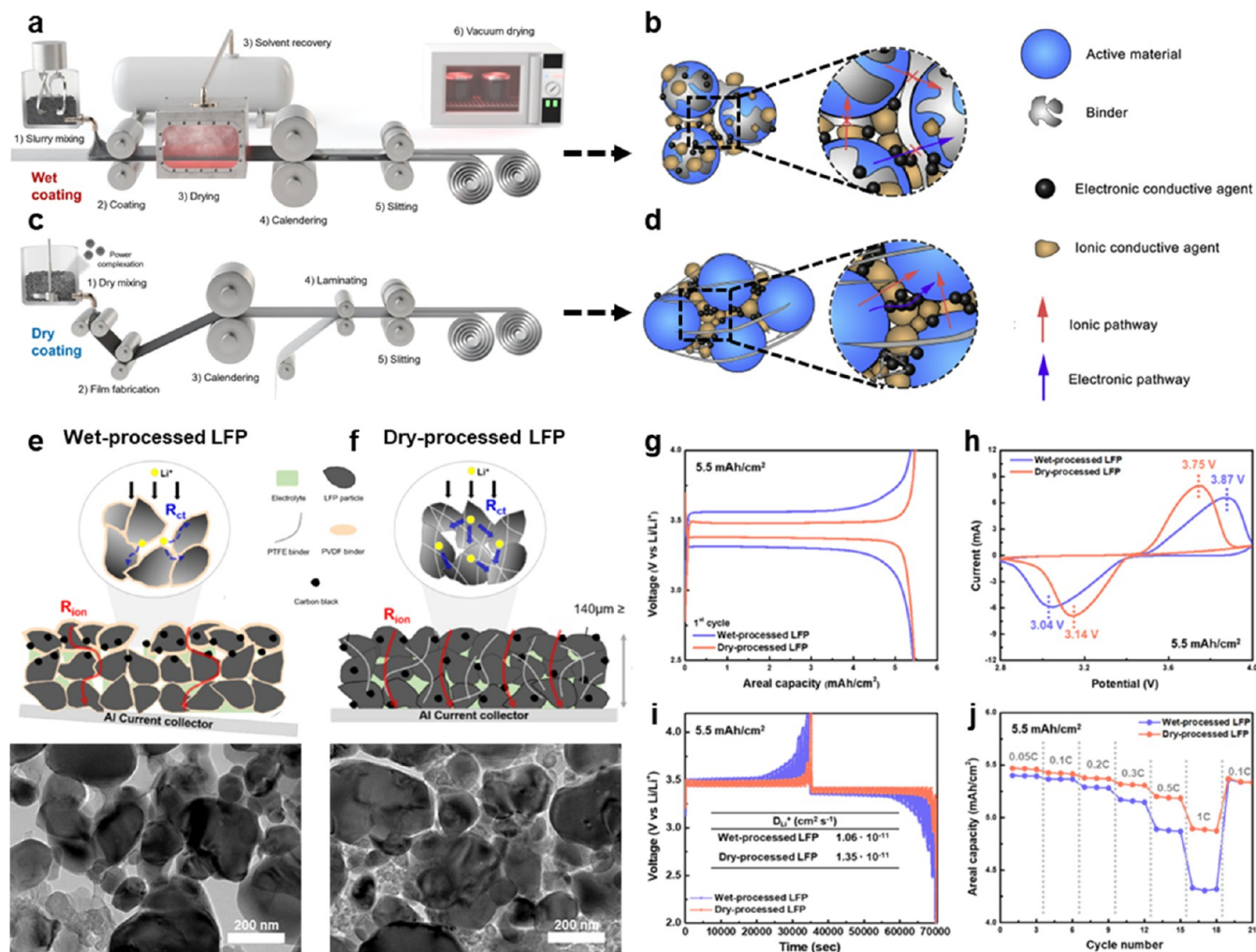
Figure 14. Comparison of wet- and dry-processing for electrode fabrications. (a, c) Schematic illustrations of conventional slurry-based wet coating and solvent-free dry coating, respectively. (b, d) Conceptual diagrams of particle-level connections in the two processes, showing differences in electronic and ionic pathways. (e, f) Cross-sectional and microstructural images of dry-processed LFP electrodes, demonstrating compact architecture and efficient ion transport networks. (g–j) Electrochemical characterization of wet- and dry-processed LFP electrodes with high areal mass loading of 5.5 mAh cm -2 , including first cycle voltage profiles (g), Cyclic voltammetry profile showing lower cell overpotential of dry-processed LFP electrode (h), Li + -ion diffusion coefficient from GITT (i), and superior rate performance. Panels are reproduced with permissions from a and c, ref 291, © 2024 Wiley-VCH GmbH, CC-BY 4.0; b and d, ref 292, © 2022 Elsevier; e–j, ref 293, © 2024 Wiley-VCH GmbH, CC-BY 4.0.
